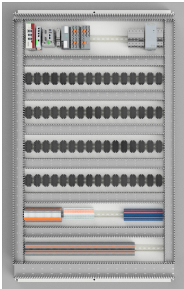
PLC Control Panel- 3D back panel layout
